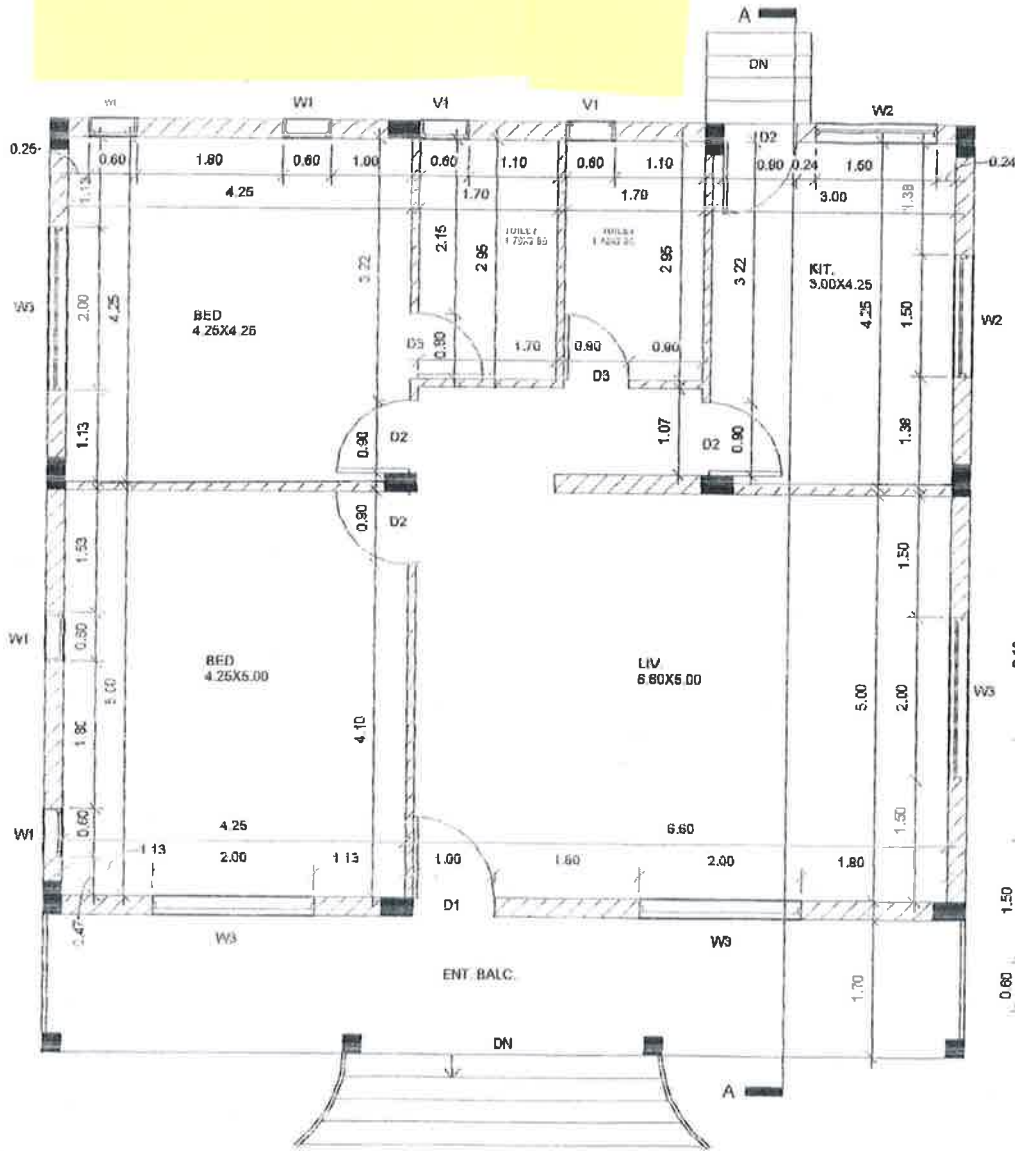
GROUND FLOOR WORKING DRAWING
